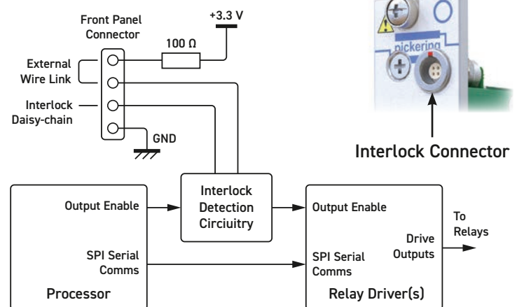
Interlock Signal Routing Diagram for 40/42-230
