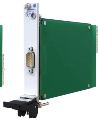
42-230 High Voltage Resistor Module in PXIe Format
