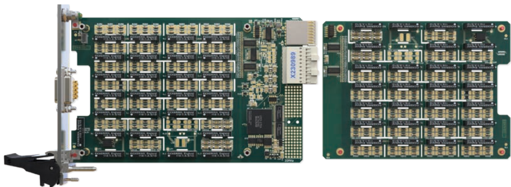
View showing Mother & Daughter cards of the High Voltage Resistor
