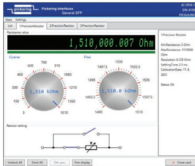
Soft Front Panel for Programmable Resistor Modules
