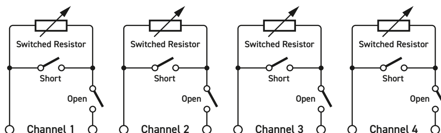
Functional Diagram for the 40/42-230 High Voltage Programmable Resistor Module - Available with 1, 2 or 4 Channels
